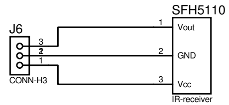
IR-RECEIVER
